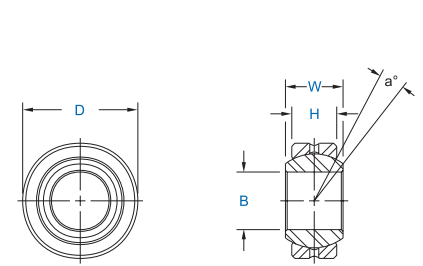
Spherical Bearing
